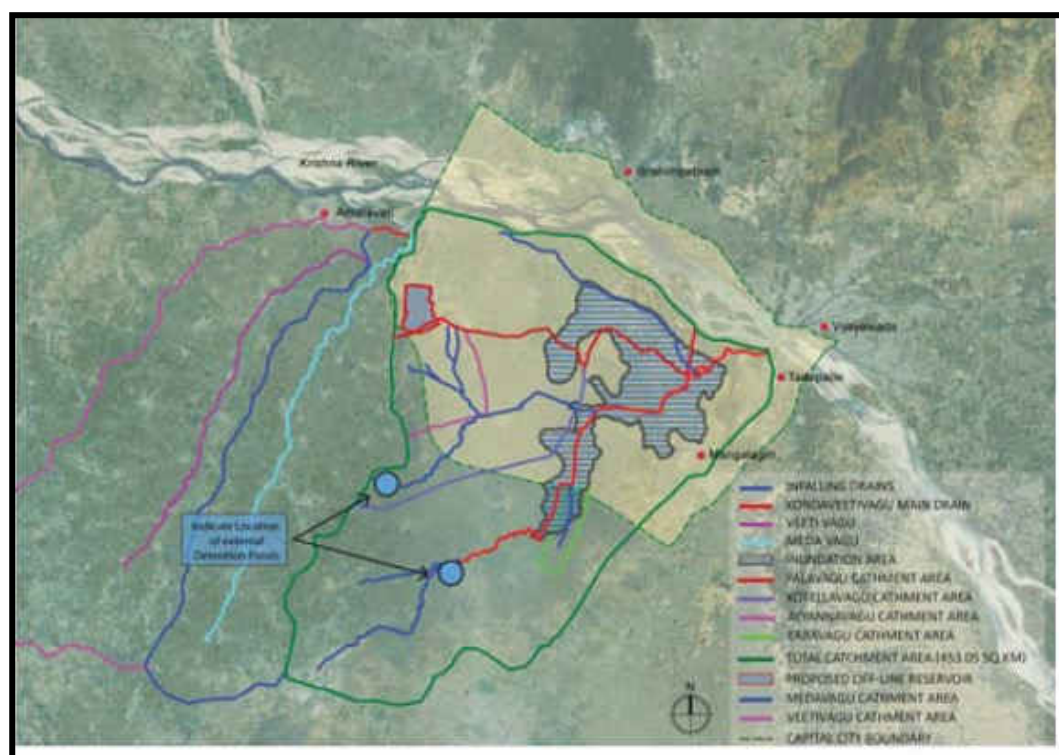
Figure 4-6 Storm-water in External Detention Ponds*
