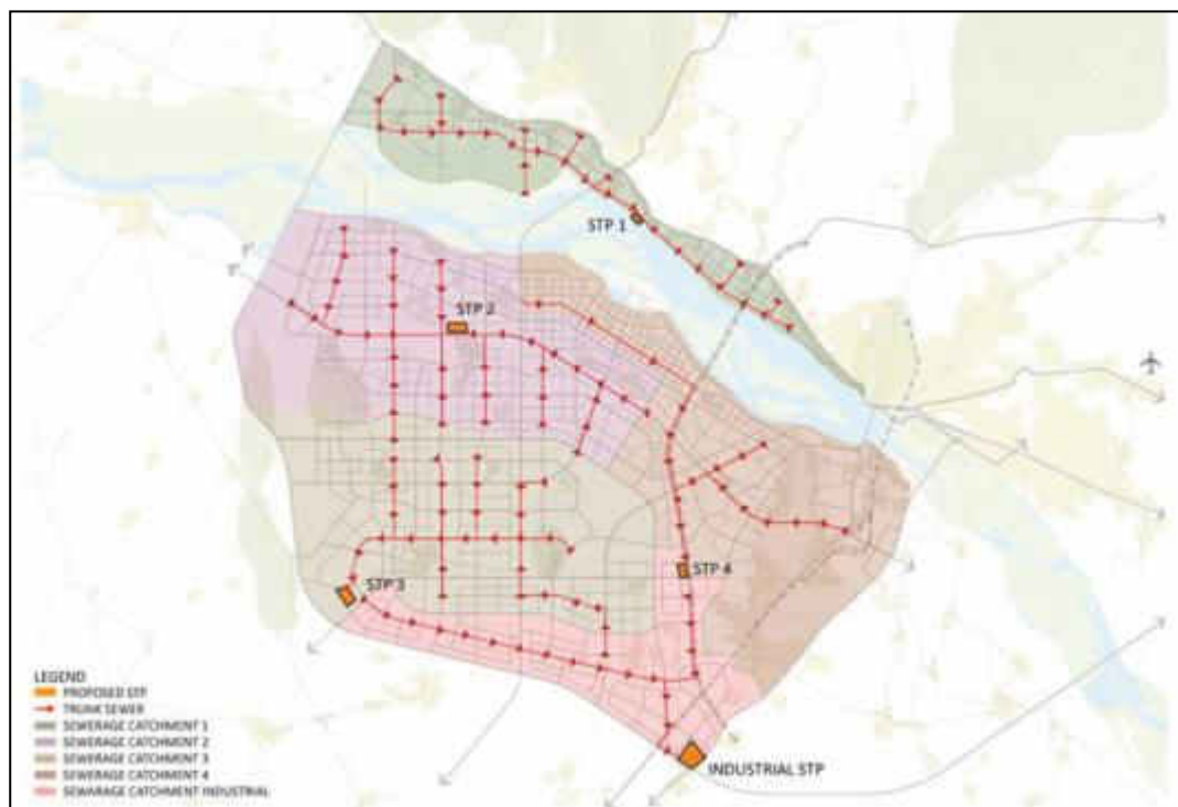
Figure 4-11 Decentralized Waste Water Management System*
